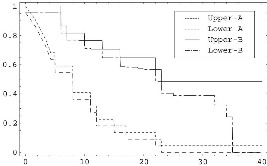
Figure 3.6: The upper and lower survival functions with ties (Example 9).
