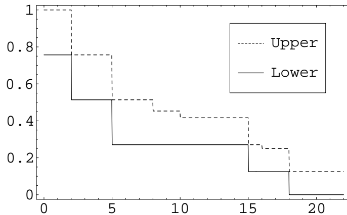
Figure 3.7: The upper and lower survival functions for T_8 (Example 10).
