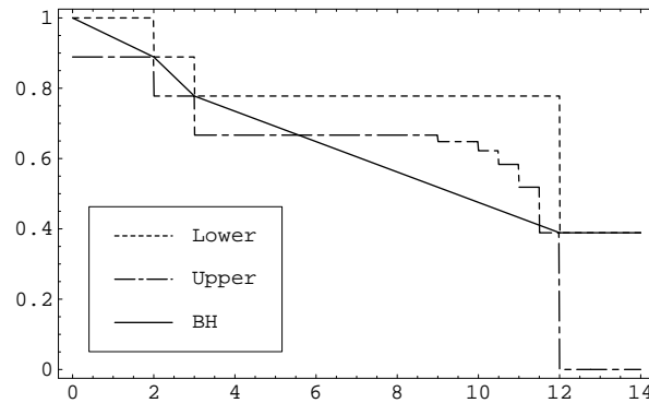
Figure 3.3: Lower and upper survival function, and the uniform BH survival function (Example 3).
